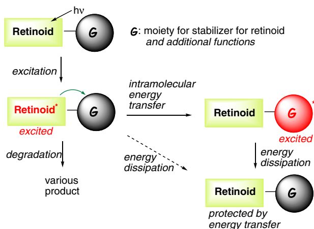
Scheme 1. Schematic explanation of internal energy transfer to the modifying group G for stabilization of retinol.
