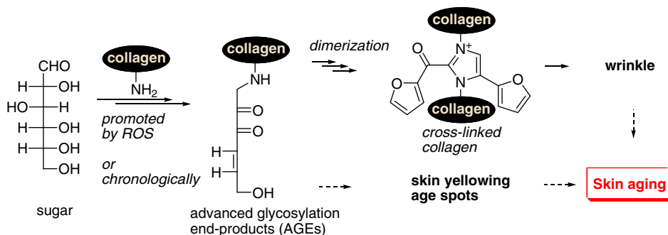
Scheme 2. Generation of AGE and cross-linked collagen by reactive oxygen species.
