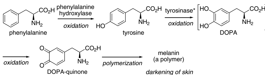
Scheme 3. The route to melanin by three consecutive oxidation reactions and polymerization starting from phenylalanine.
