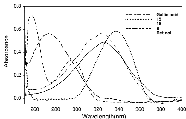
Figure 3. UV spectra of retinoids (concentration: 2.5 \times 10^{-4} M (MeOH)).
