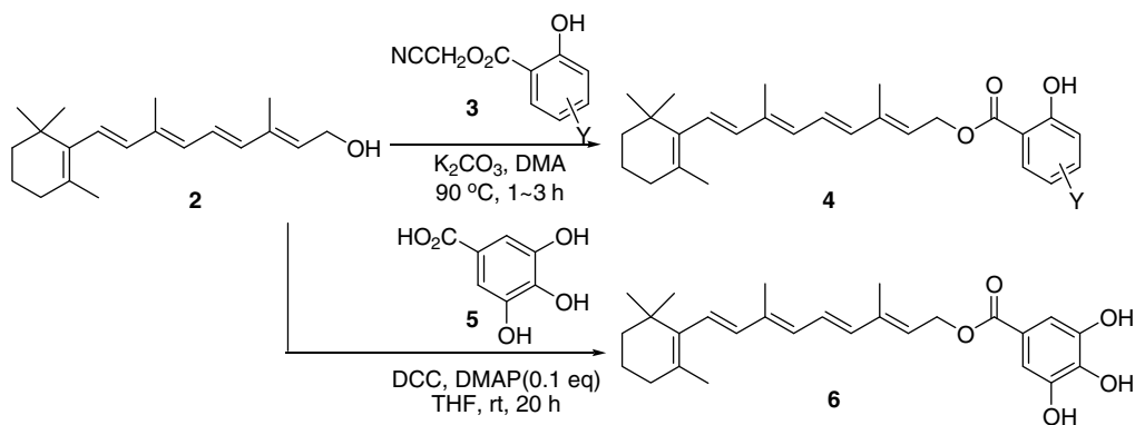
Scheme 5. Preparation of retinyl polyhydroxybenzoates.
