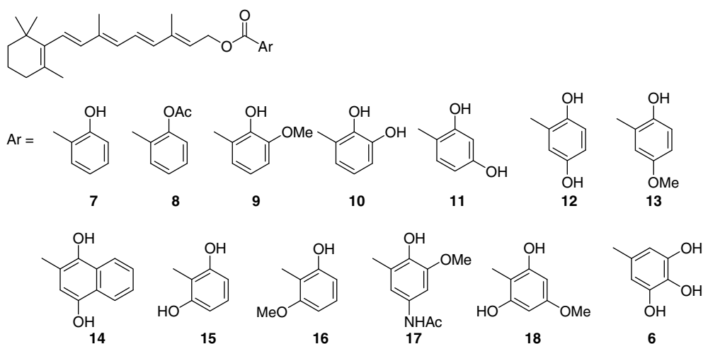
Figure 1. Representative retinyl polyhydroxybenzoates prepared in this study.
