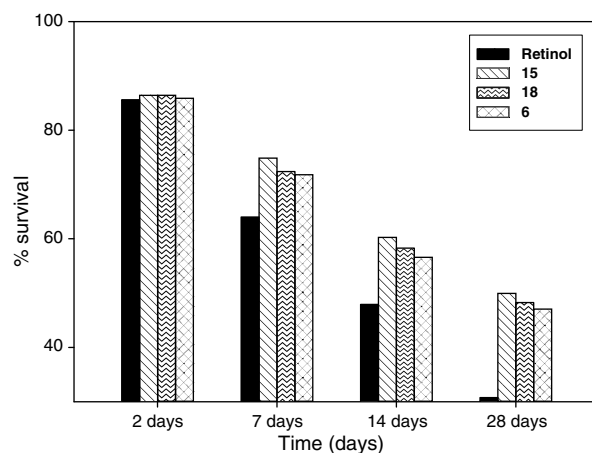
Figure 2. Thermal stability test at 40 °C.
