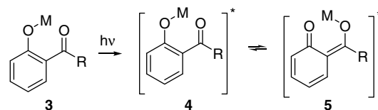
Scheme 4. Energy dissipation by excited-state intramolecular transfer of proton and metal.
